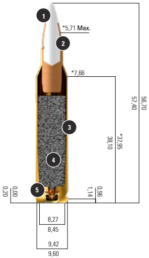
SAT IMPROVED PERFORMANCE CROSS-SECTION
